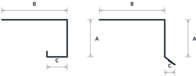
One-piece cover, hemmed return Cover with kick-out drip
